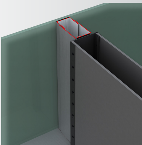
WALL-TO-GLASS
