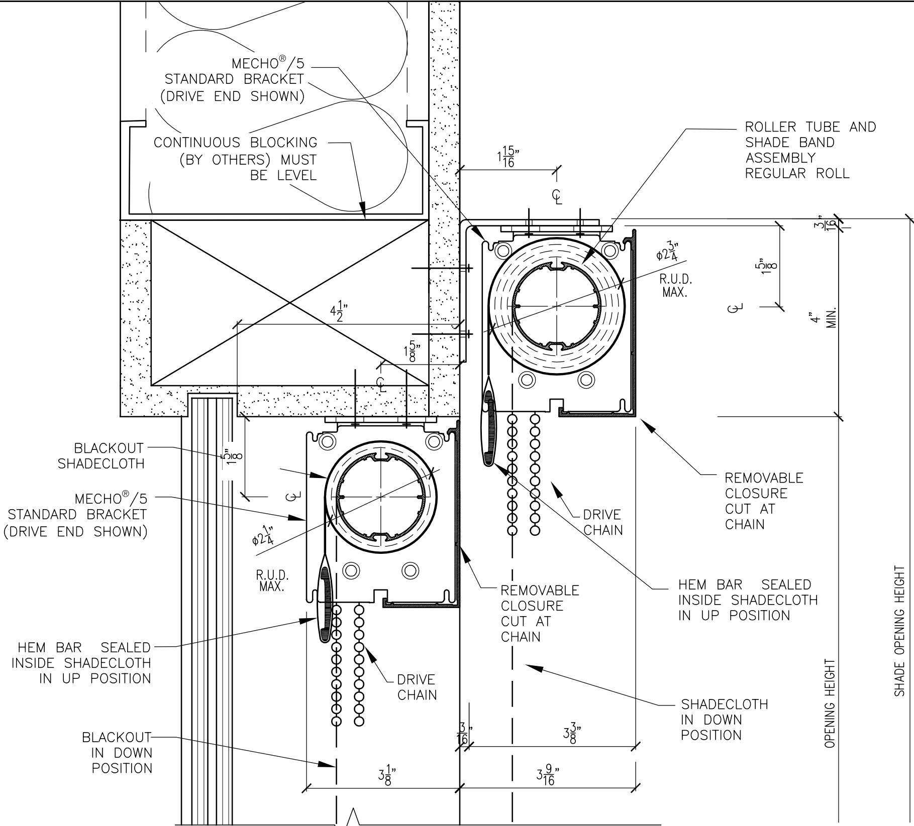
1 SECTION AT WINDOW HEAD SCALE: 6"=1'-0"
