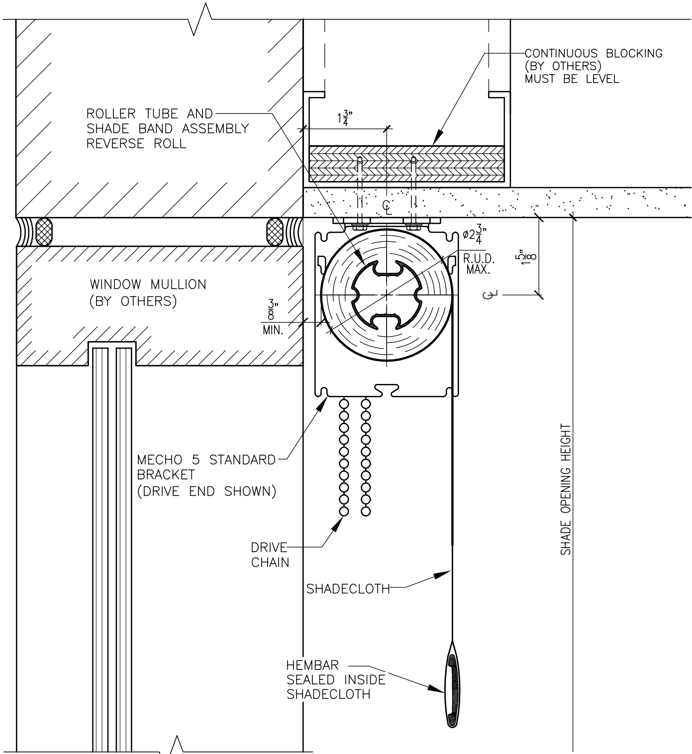
1 TYPICAL SECTION SCALE: 1/2 FULL SIZE
