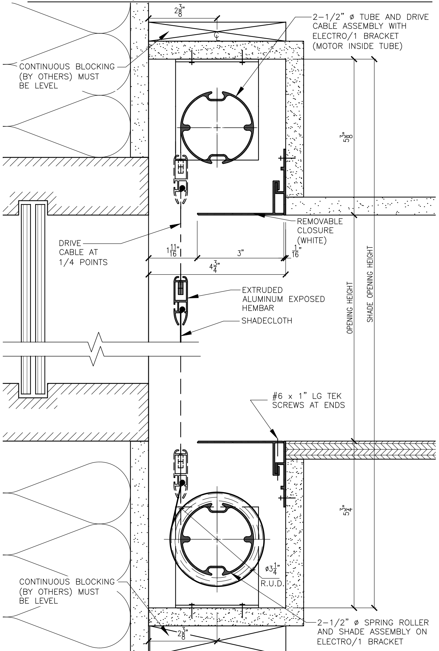
1 TYPICAL SECTION SCALE: 1/2 FULL SIZE
