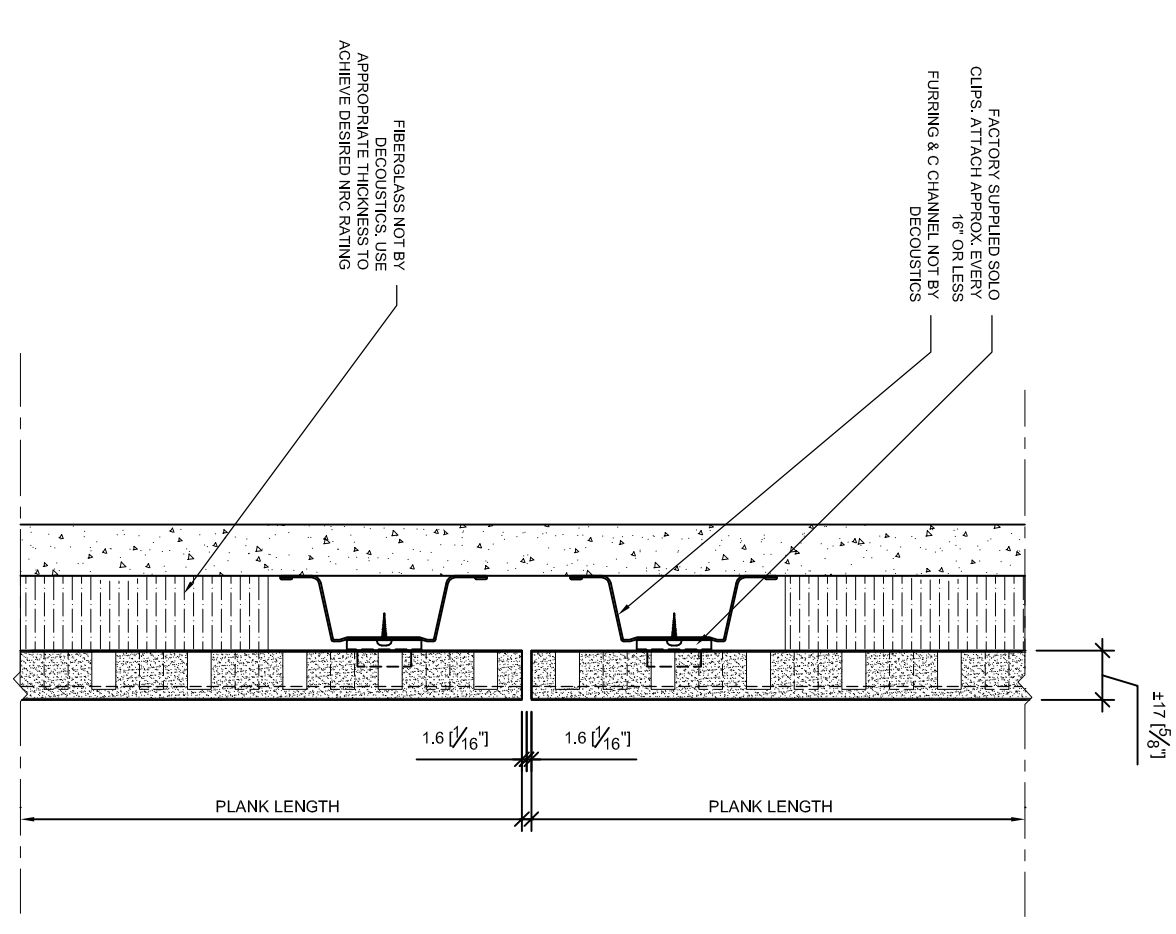
DETAIL @ DEFINED JOINT (BETWEEN 2 PLANK LENGTHS) SCALE: 1/2
